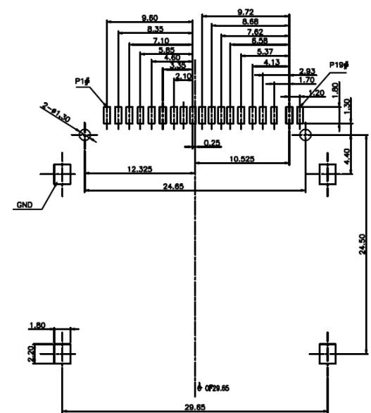
RECOMMEENDER PCB LAYOUT TOLERANCE UNLESS OTHERWISE IS ±0.05
