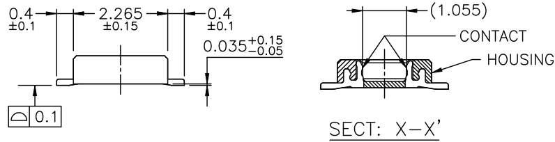
MATED DRAWING(REF.)
