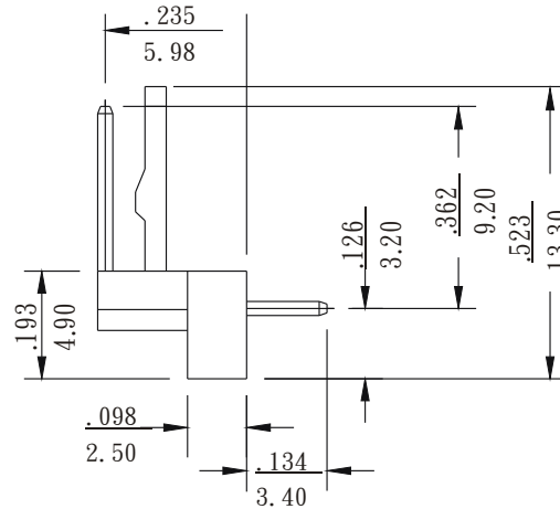
Dimensional information -inch/mm (8812/8813)
