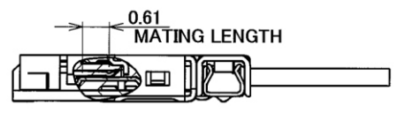
MATING CONDITION
