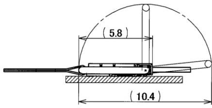
PULL-BAR MOVEMENTS
