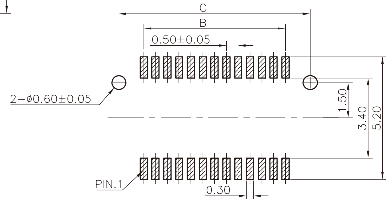
PCB LAYOUT
