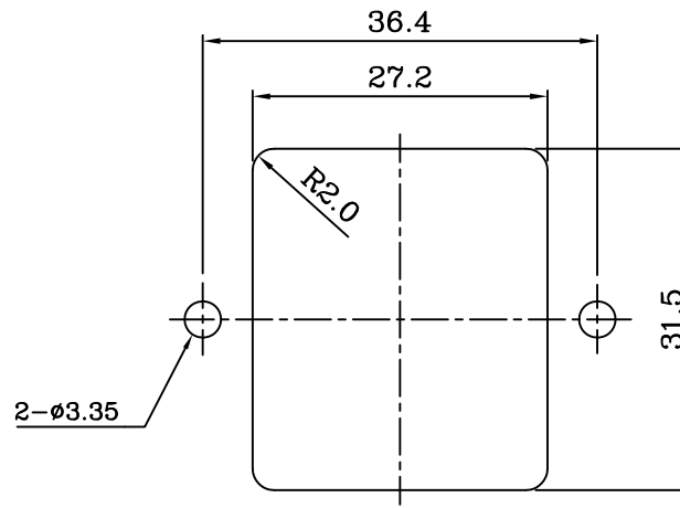
PANEL CUT-OUT
