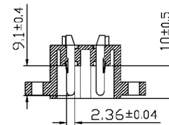
SECTIONAL
