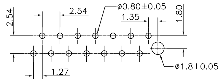
PCB Layout
