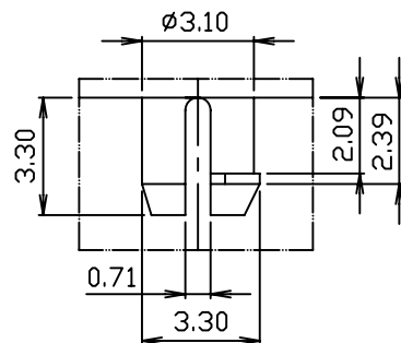
DETAIL X
