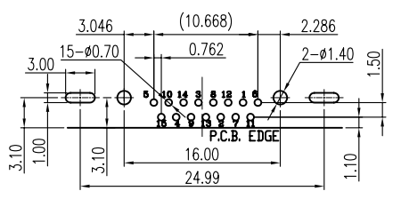
RECOMMENDED P.C.B LAYOUT INSPECTION DIMENSION:(A)~(K)
