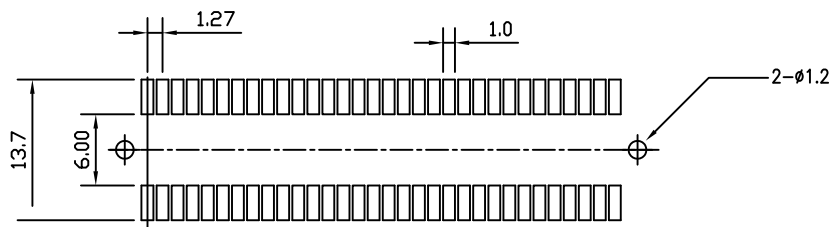
RECOMMENDED PCB LAYOUT (TOP VIEW)
