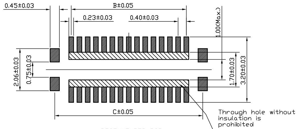
RECOMMENDED PCB PATTERN
