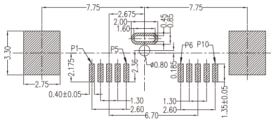
PCB LAYOUT(T=1.00mm) COMPONENT SIDE
