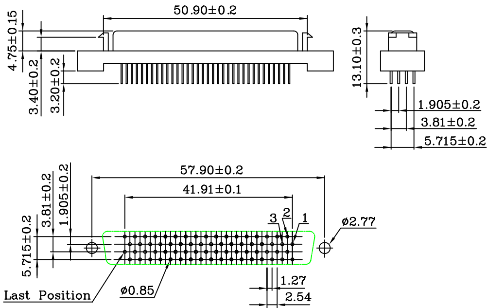
PCB Layout (B)
