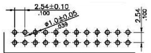
Recommmand PCB Layout
