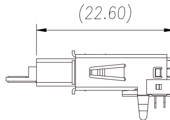
MATING DIAGRAM SCALE 2 : 1
