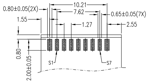
P.C.B. LAYOUT(T=1.00mm) COMPONENT SIDE
