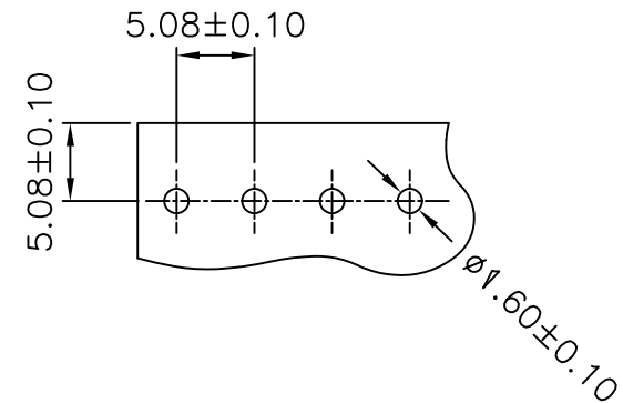
Recommended Hole Dimensions
