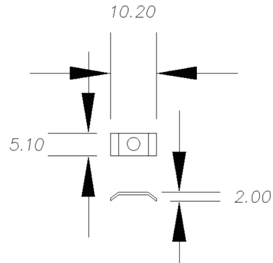
square washer for shoulder screw
