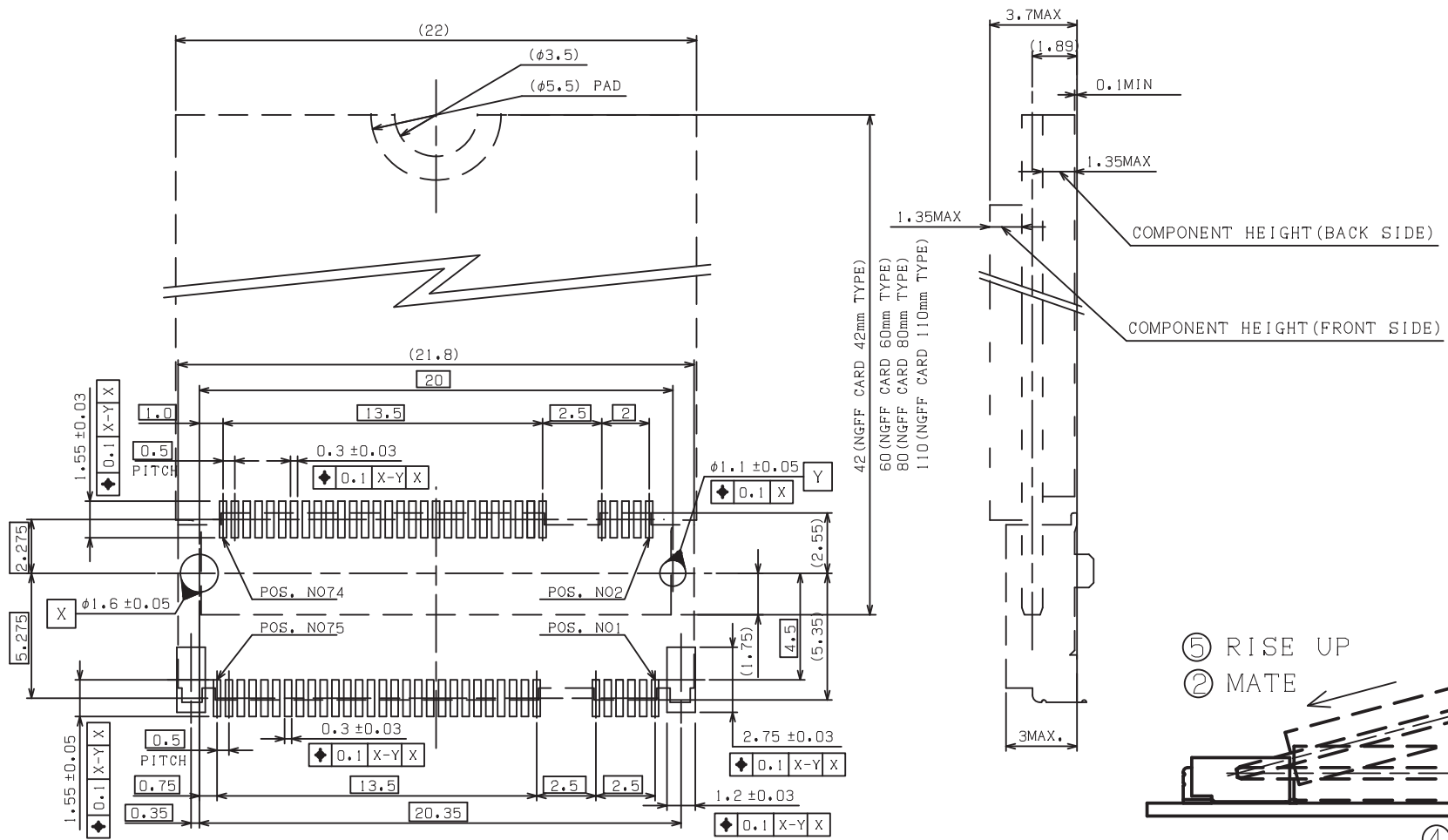
KEY ID "B" RECOMMENDED P.C.B. BOARD LAYOUT
