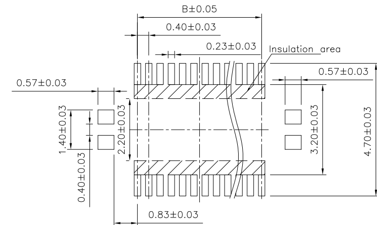
PCB Layout
