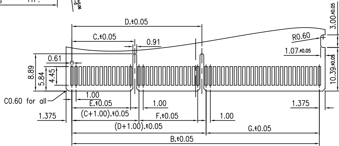
RECOMMENDED CARD PCB LAYOUT
