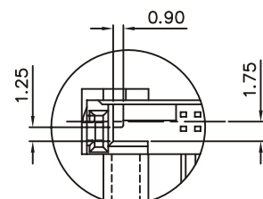
A VIEW S=2/1 FOR 5.0 V
