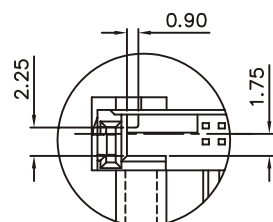
A VIEW S=2/1 FOR 3.3 V
