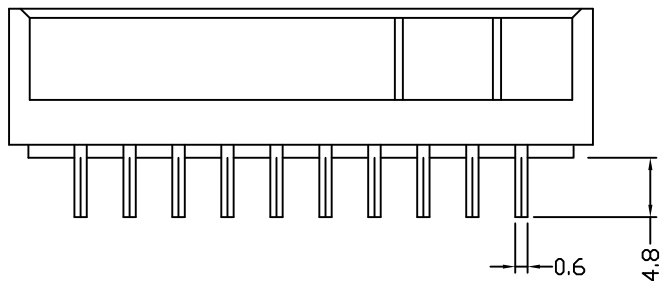
DIP TYPE
