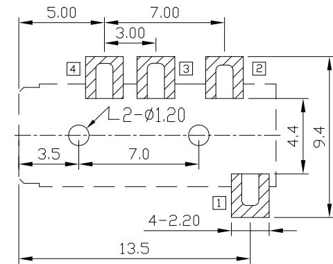
RECOMMENDED SOLDER PAD LAYOUT ( \pm 0.1 )
