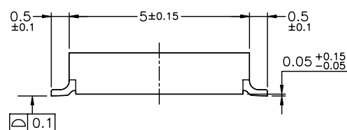
MATED DRAWING(REF.)
