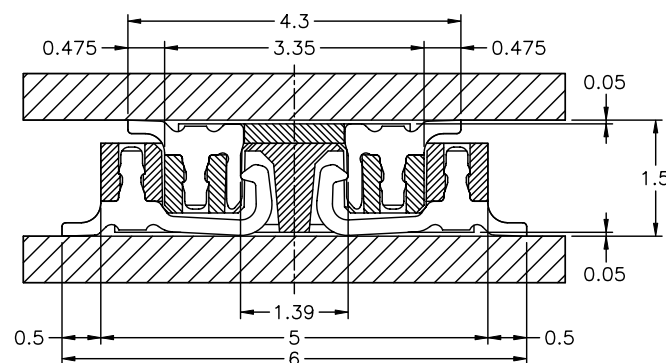
MATED DRAWING(REF.)
