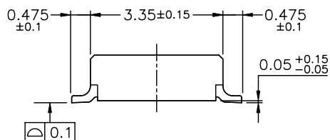
MATED DRAWING(REF.)
