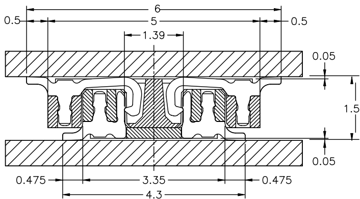
MATED DRAWING(REF.)
