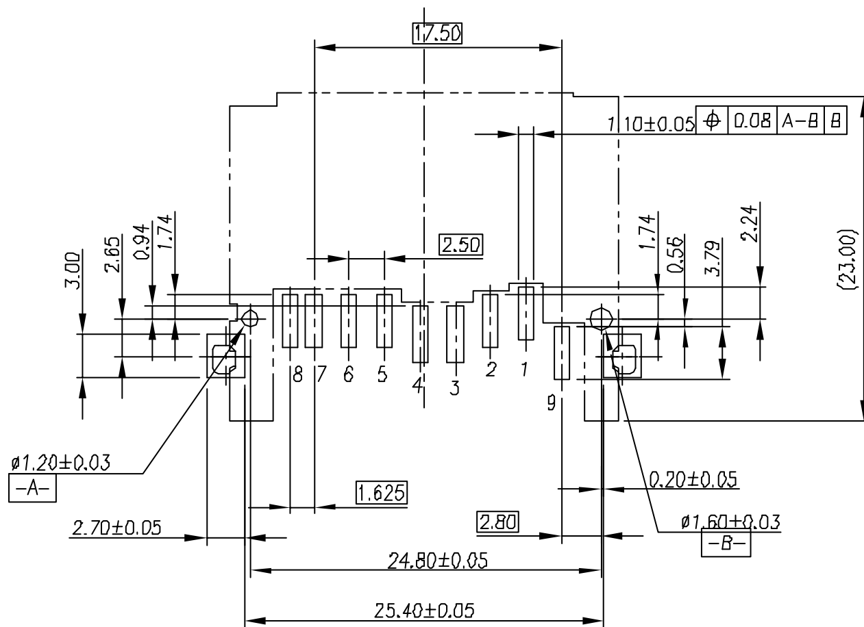
PC BOARD LAYOUT COMPONENT SIDE
