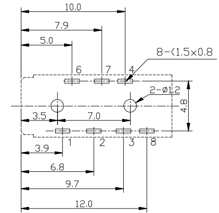
REFERENTIAL DIMENSIONS OF PC BOARD HOLES (TOLERANCE/ALL±0.1)(PRINTED-SIDE VIEW) T=1.6 TOP VIEW
